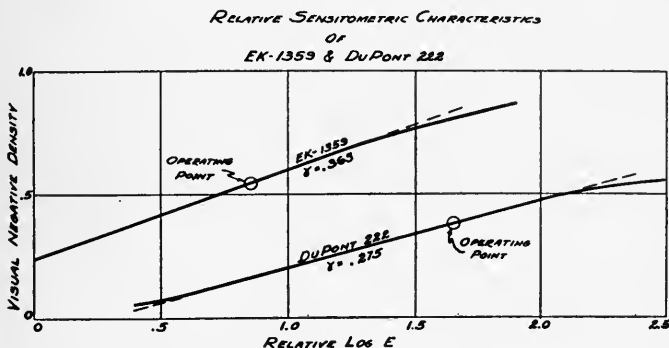
FIG. 7. IIb sensitometric characteristics of (a) EK-1359 in normal negative sound developer; (b) Dupont 222 fine-grain in special negative sound developer.
